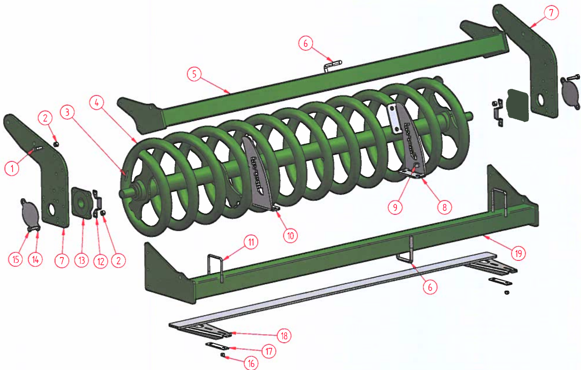
RULLO SPIRALE - SPIRAL ROLLER
