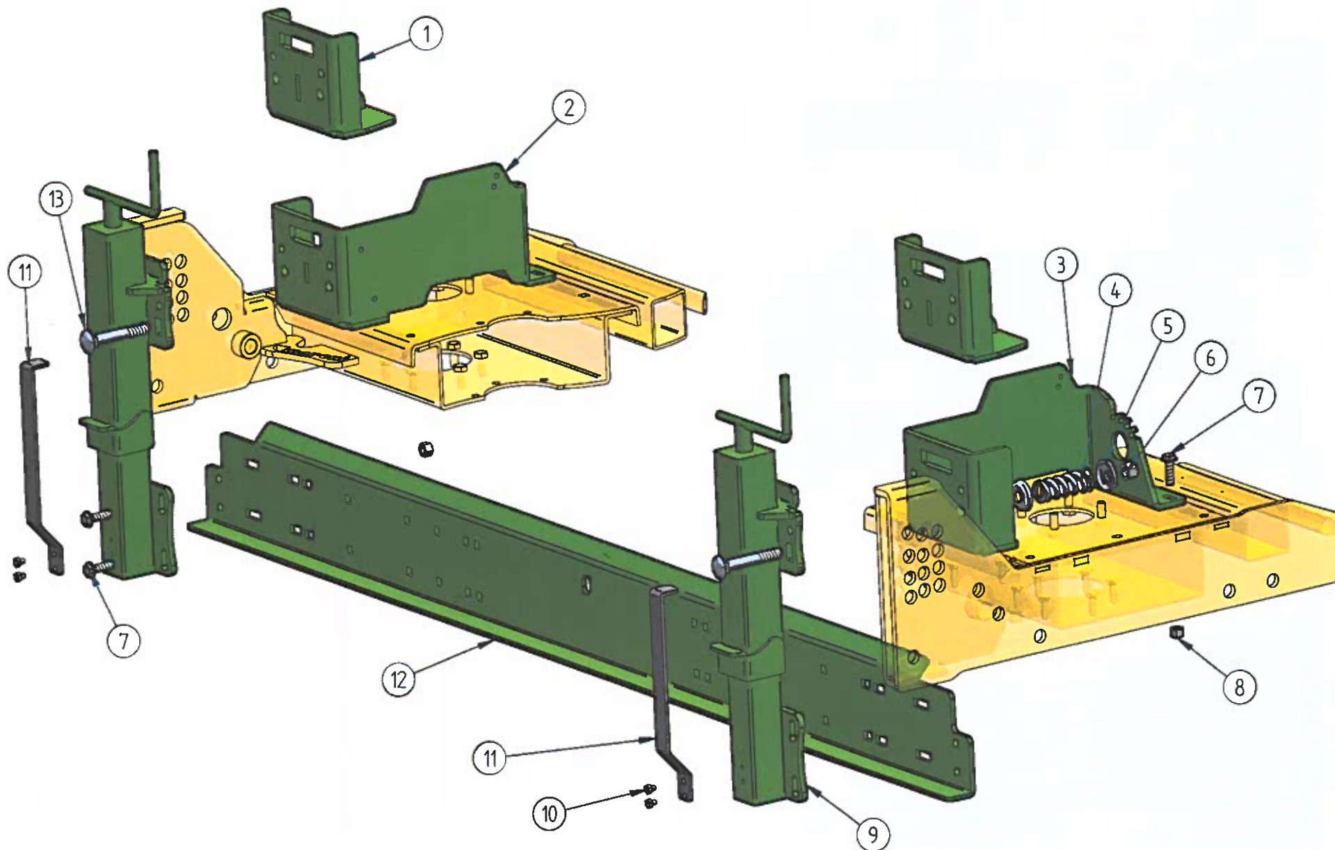
BARRA POSTER. ERPICI FISSI - BAR HANDLE'S CONNECTION
