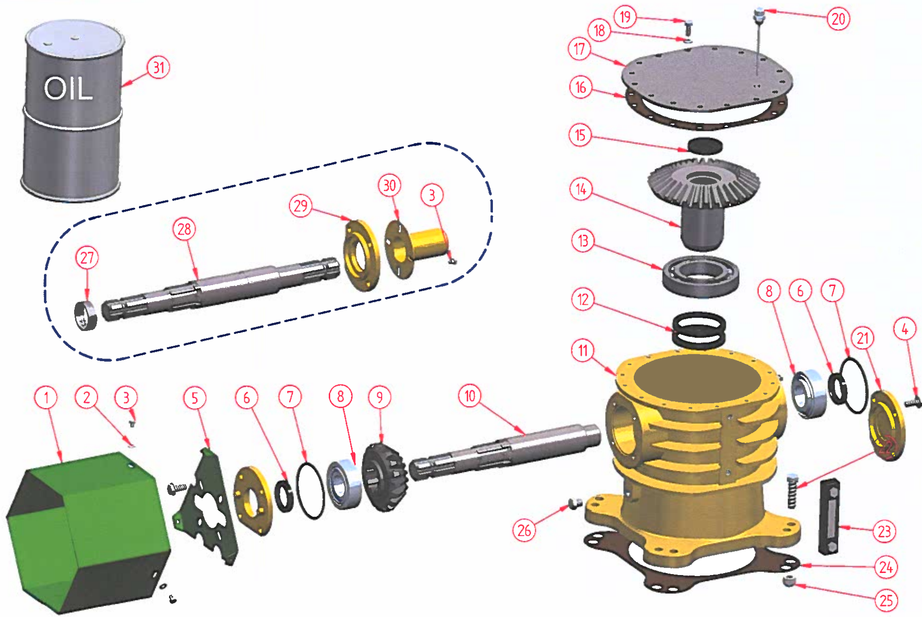
RIDUTTORE MONOVELOCITA' - SINGLE SPEED GEARBOX
