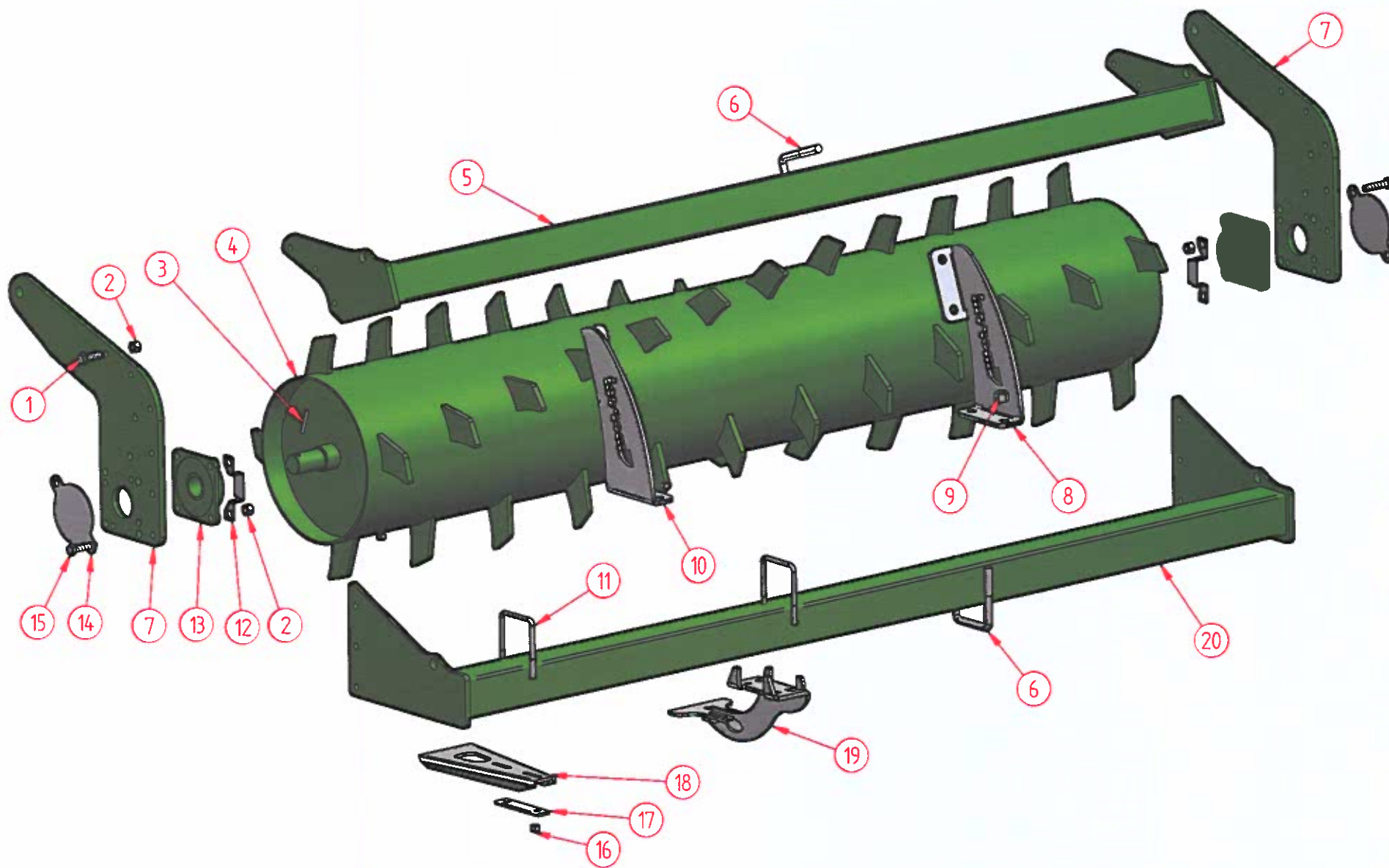
RULLO RISAIA - PADDY FIELD ROLLER
